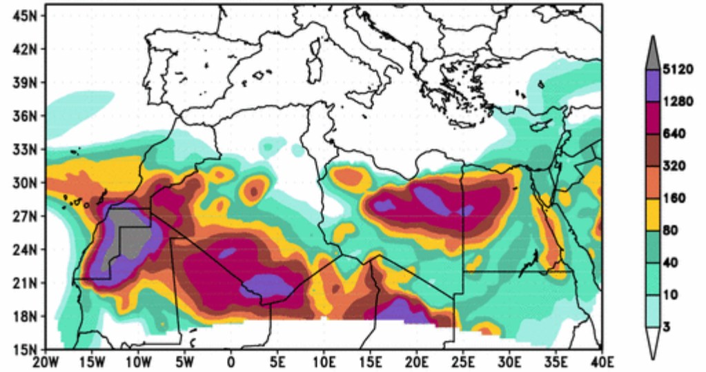
ICoD/DREAM Lowest Model Level Dust Concentration ( \mu\text{g}/\text{m}^3 ) 30h forecast for 18z 17 JAN 05
